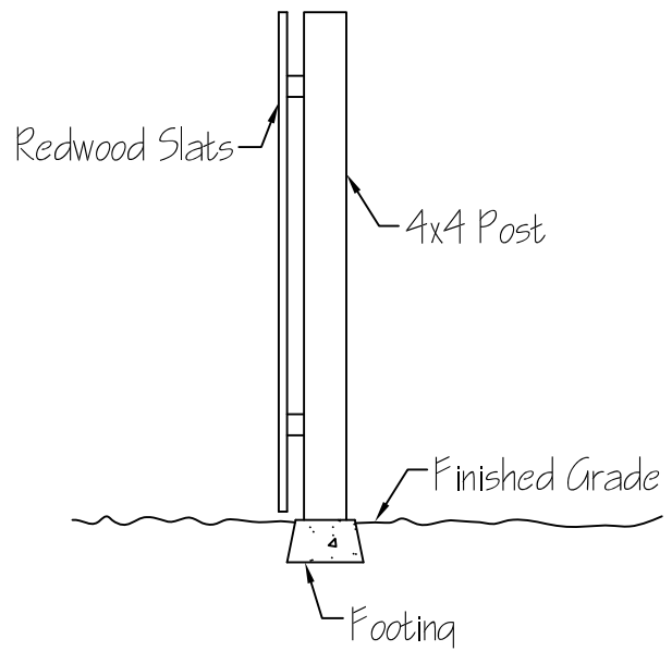
Section (Show Materials)
