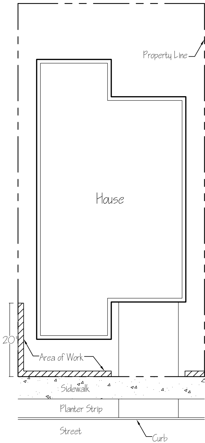
Site Plan (Show Area of Work)
