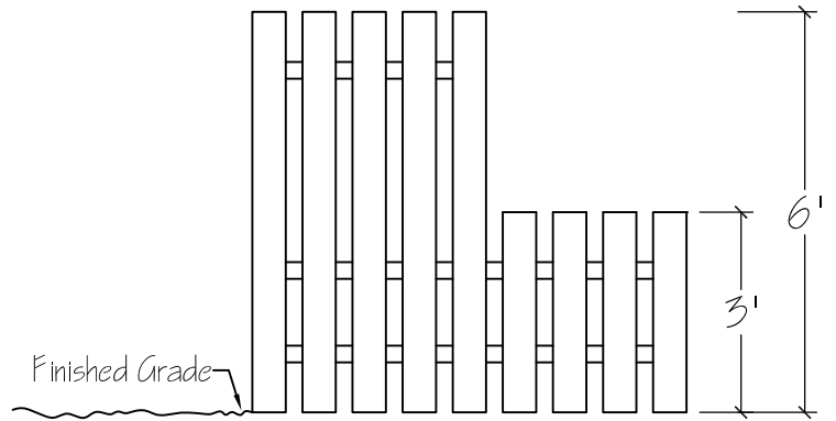
Elevation (Show Height)
